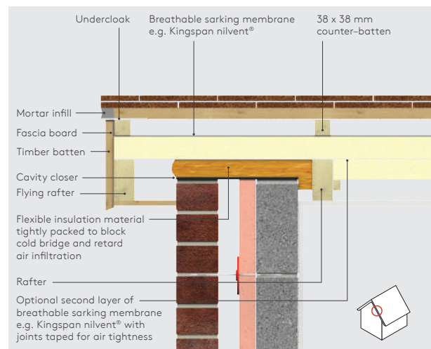
Figure 7c - Eaves detail
